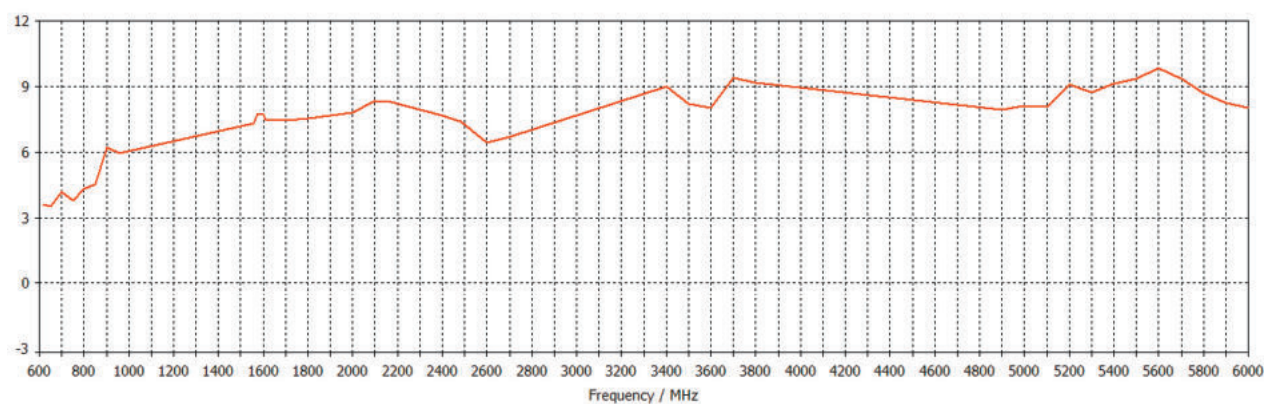
Typical Peak Gain - 4G/5G Elements*
