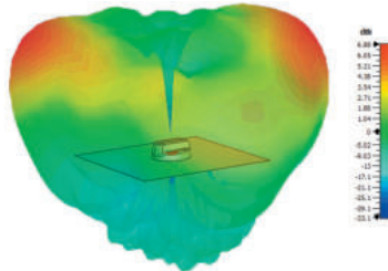
Typical 3D Pattern - 4G/5G Elements 1800MHz
