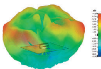
Typical 3D Pattern - 4G/5G Elements 3600MHz
