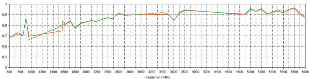
Typical Peak Gain - 4G/5G Elements*
