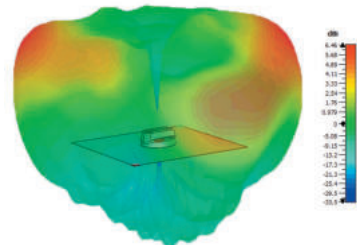
Typical 3D Pattern - 4G/5G Elements 2000MHz
