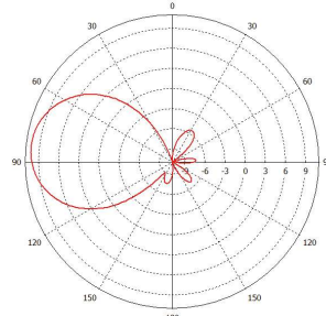
Typical E Plane (3600MHz)
