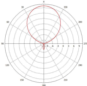
Typical H-Plane (3600MHz)
