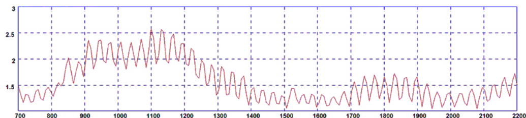
Typical VSWR*
