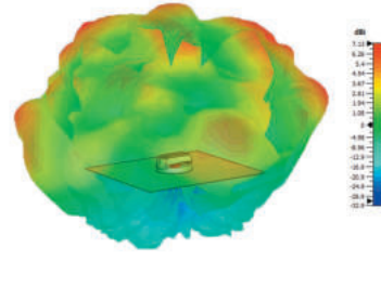
Typical 3D Pattern - 4G/5G Elements 5400MHz
