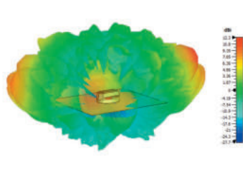
Typical 3D Pattern - WiFi Elements 5400MHz
