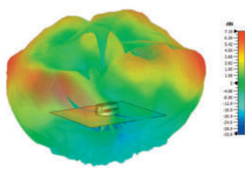
Typical 3D Pattern - 4G/5G Elements 3600MHz
