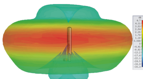
Typical 3D Plot (5400MHz)
