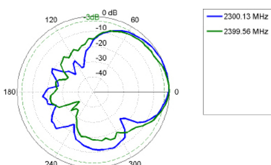
Elevation: 2300 – 2400 MHz
