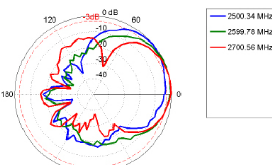
Elevation: 2500 – 2700 MHz
