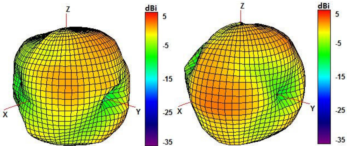
Cable 1: CELLULAR/LTE
