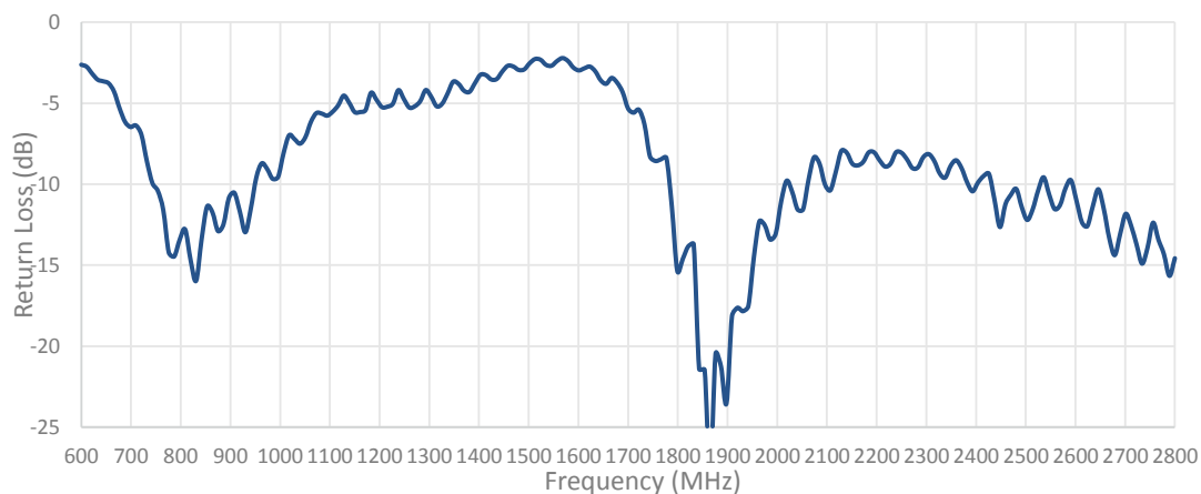
Cable 1: CELLULAR/LTE
