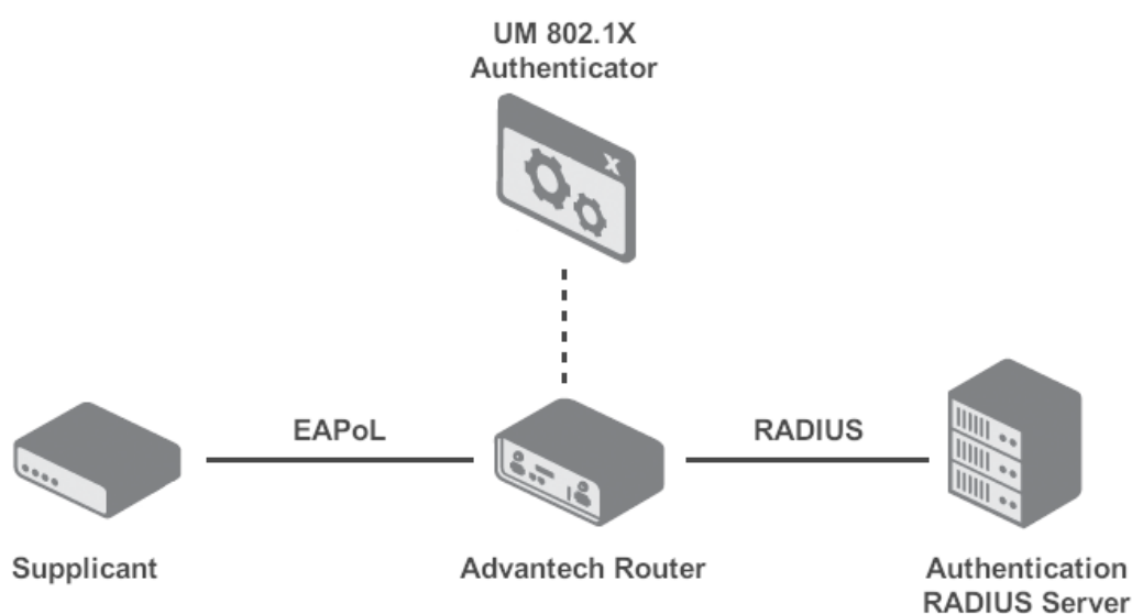
Figure 1: Functional Diagram
